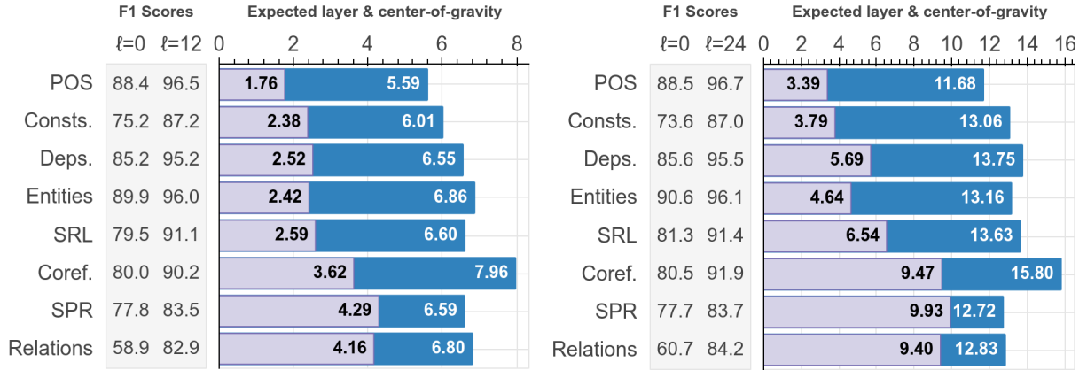
(a) BERT-base
